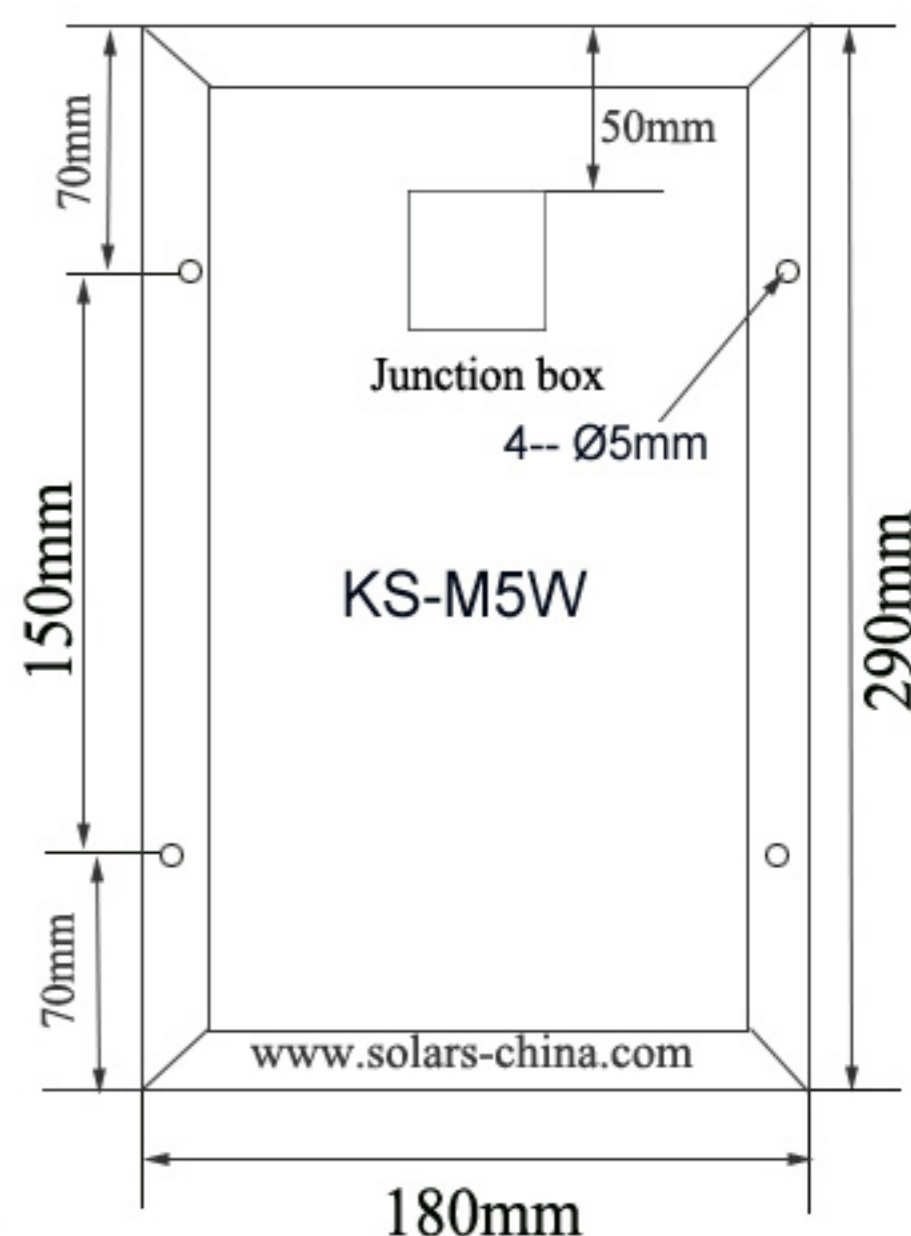
BACK VIEW
