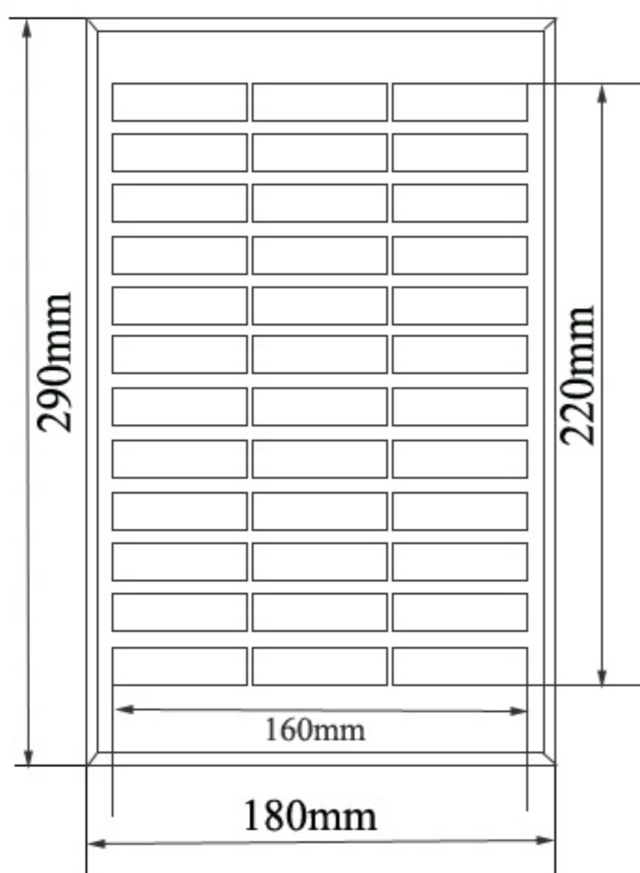
FRONT VIEW(1)
